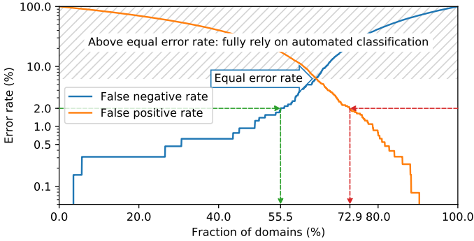
Fig. 4. FNR and FPR as a function of the fraction of domains with a score below a certain value. By choosing the maximum error rate, we determine the fraction of domains that can be automatically classified.
